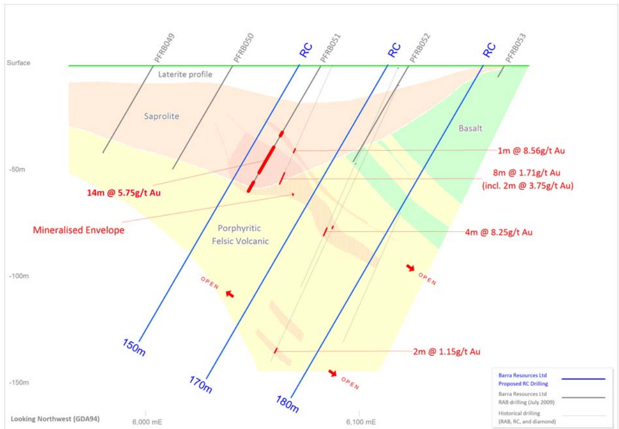
Figure 2: Schematic cross-section through Diablo showing planned RC drilling in relation to RAB drill hole PFRB051.
